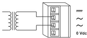
AC Powered
